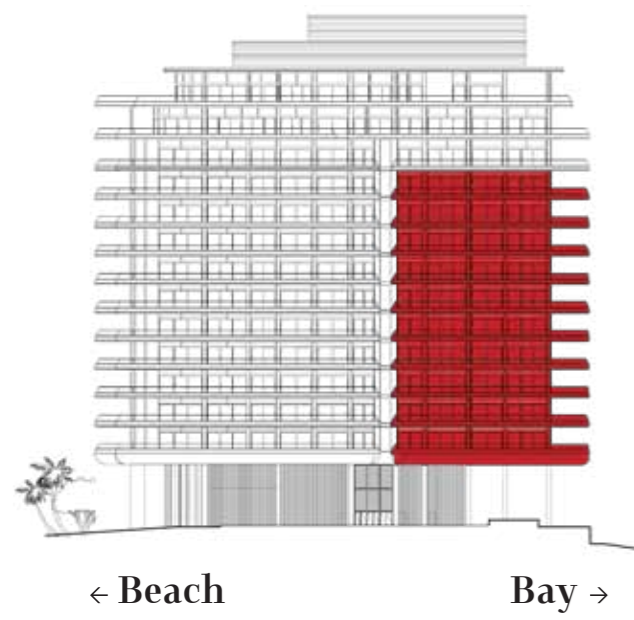
NORTH FACADE
